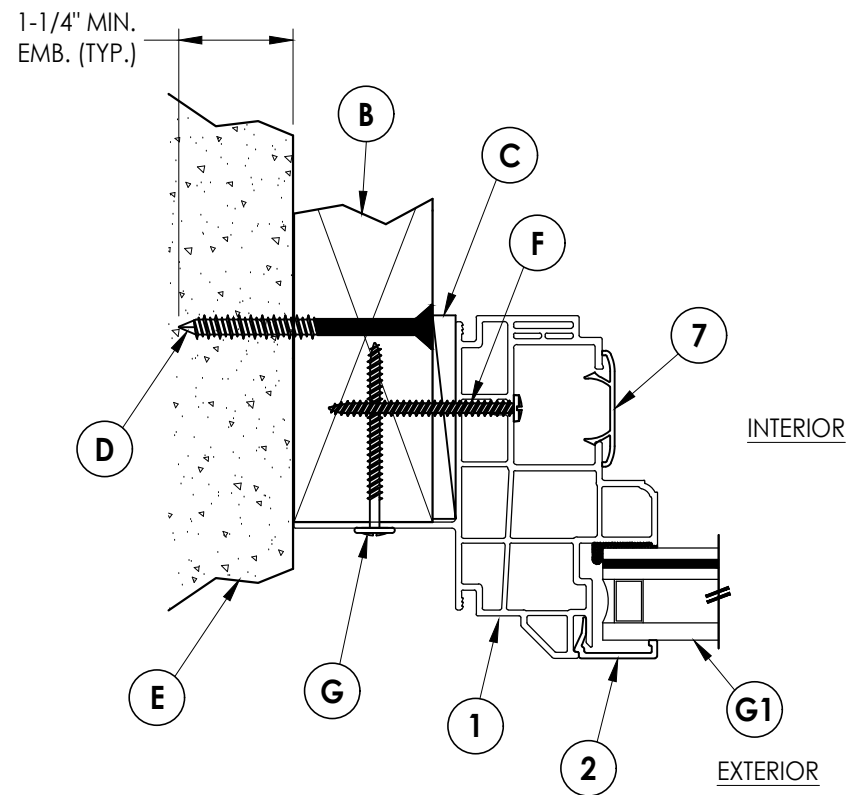
1 HORIZONTAL CROSS SECTION 2 Shown w/ 2X Buck Construction
