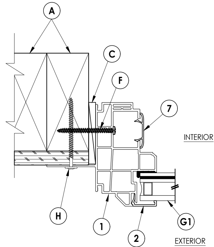
2 HORIZONTAL CROSS SECTION 2 Shown w/ Stud Construction
