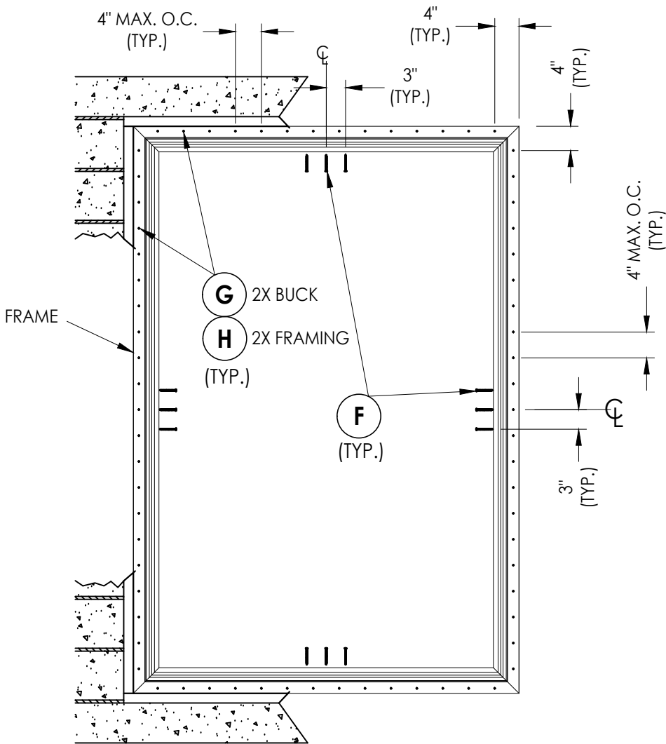
FRAME ANCHORING
